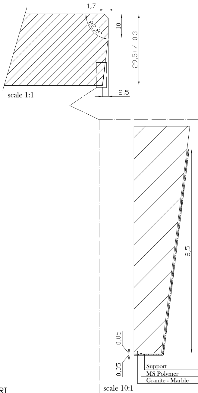
Detail of the tile edge with assembled chamber
